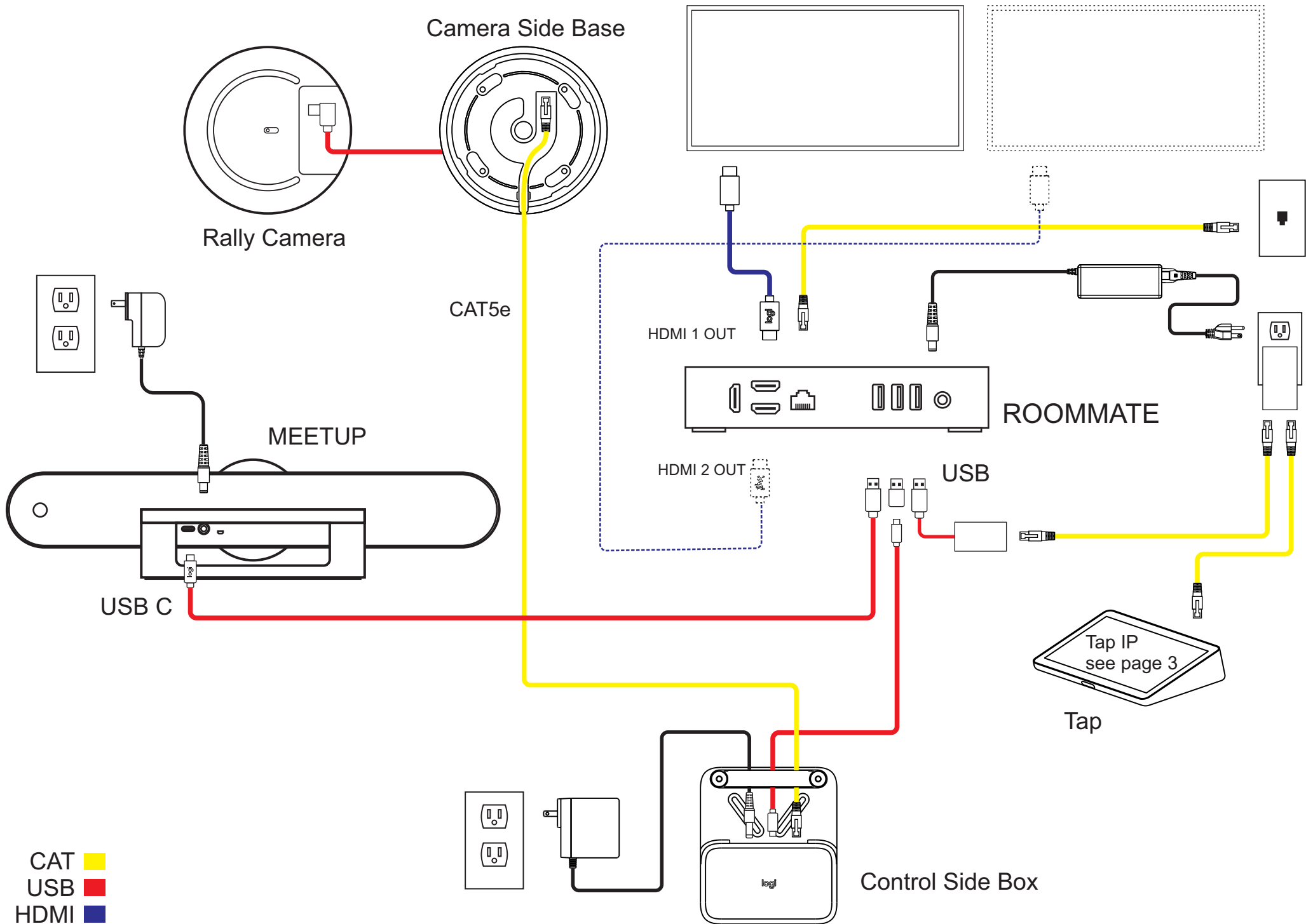
RoomMate and MeetUp with Rally Camera Streamline Kit Android Mode with Zoom Room Requires CollabOS 1.14 or later
